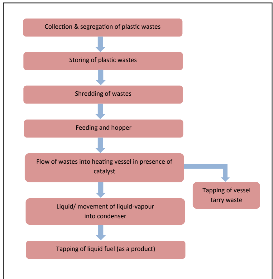
Figure 14: Typical process flow for depolymerisation
