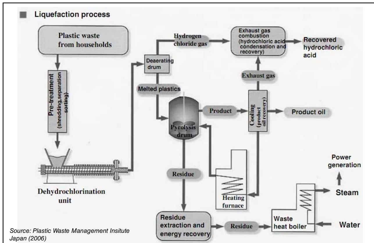
Figure 16: Typical process flow for liquefaction/blast furnace
