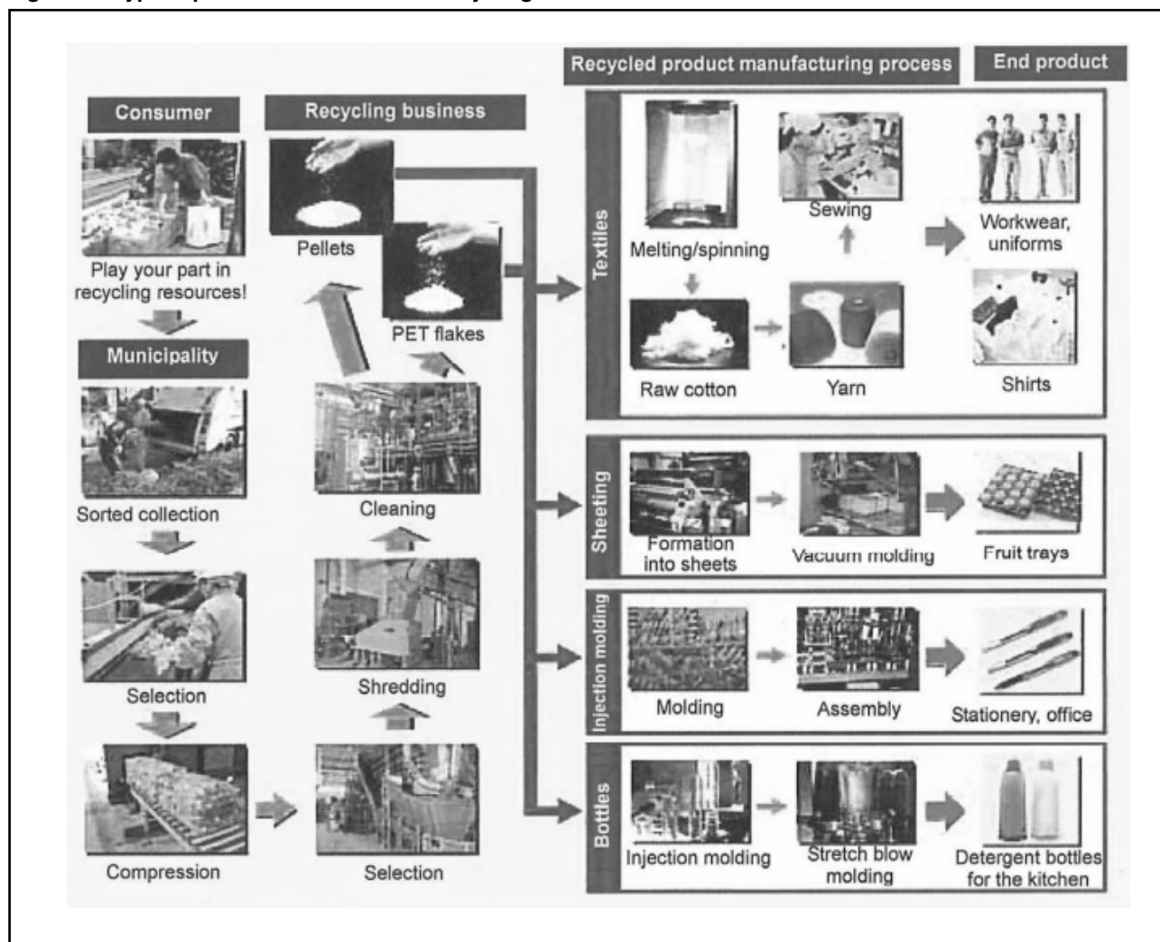
Figure 13: Typical process for mechanical recycling of PET bottles
