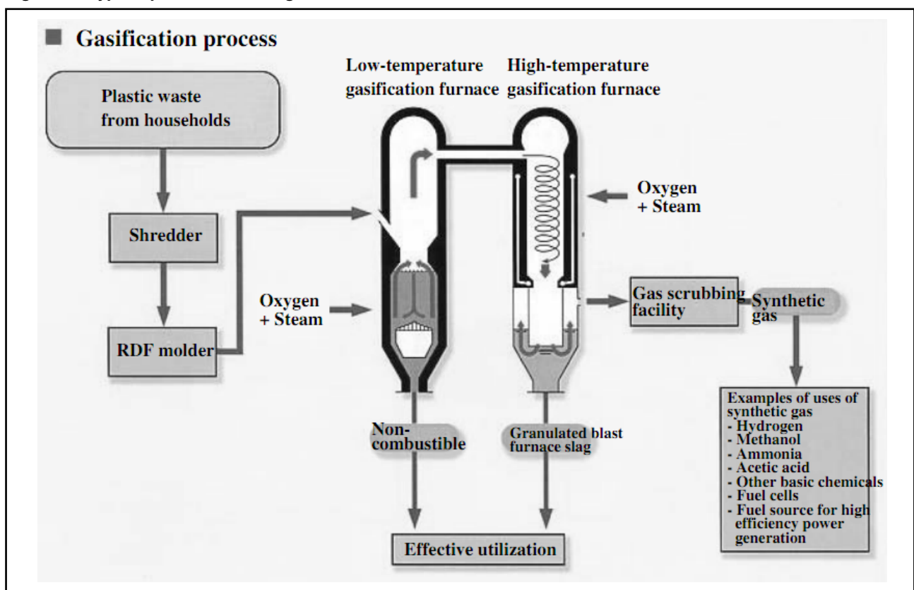
Figure 15: Typical process flow for gasification
